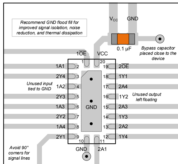
图 11-2. Example layout for the SN74HCS244-Q1 in the WRKS package
