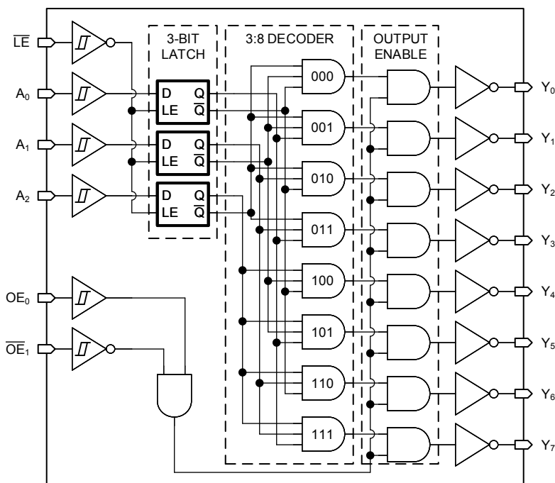
图 8-1. Logic Diagram (Positive Logic) for the SN74HCS137
