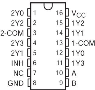
图 4-1. PW Package, 16-Pin TSSOP (Top View)
