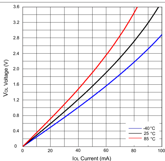
图 5-1. Low-Level Output Voltage ( V_{OL} ) vs Low-Level Current ( I_{OL} )
