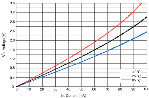
图 5-1. Low-Level Output Voltage ( V_{OL} ) vs Low-Level Current ( I_{OL} ) at V_{CCA} = V_{CCB} = 3.6V
