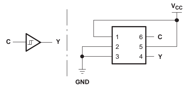
Figure 8. Noninverted Buffer
