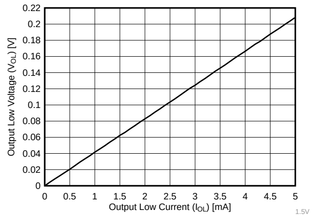
图 2. Typical Output Low Voltage of 1.5 V (25°C)
