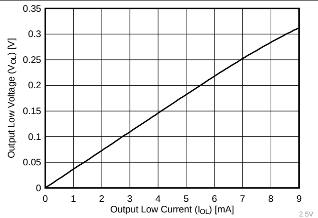
图 4. Typical Output Low Voltage of 2.5 V (25°C)
