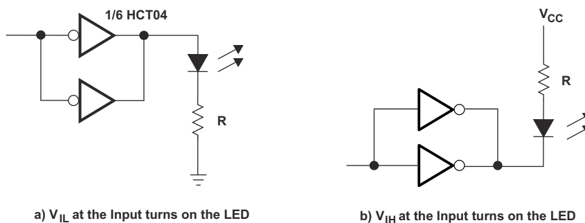
图 8-2. Driving LEDs
