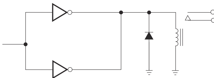
图 8-1. Driving Relays
