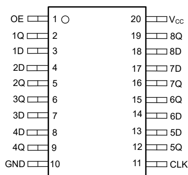
Figure 4-2. SN74AHC374-Q1 PW, DGS Package (Top View)
