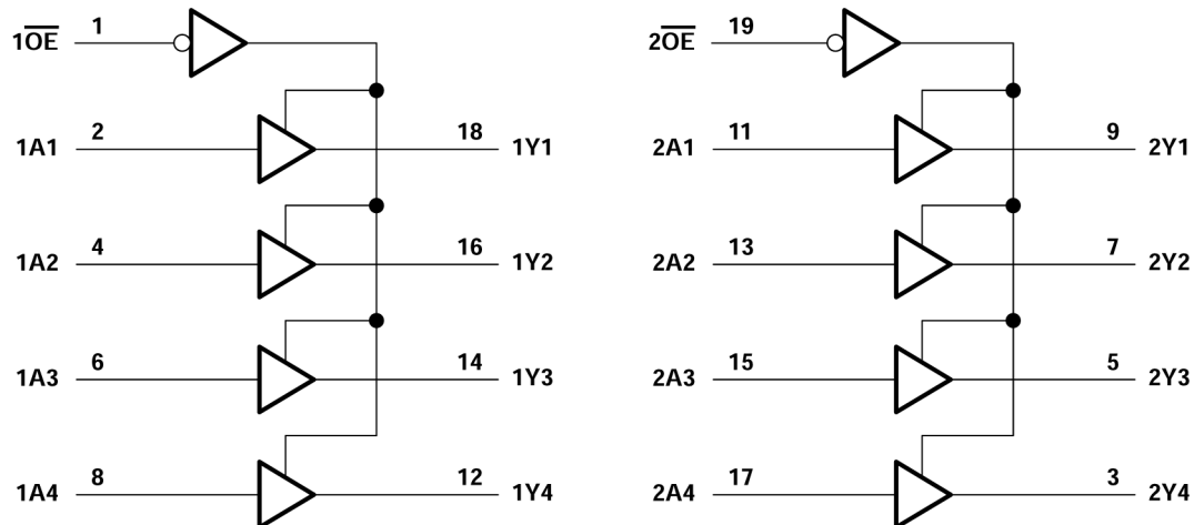
图 8-1. Logic Diagram (Positive Logic)
