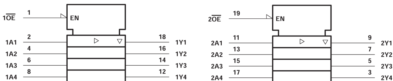
图 6-1. Logic Diagram (Positive Logic)
