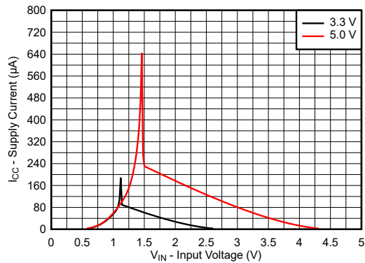
图 6-1. Supply Current Across Input Voltage 3.3-V and 5.0-V Supply
