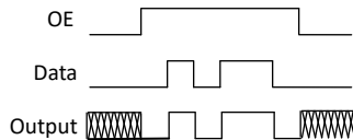
图 9-2. Application Timing Diagram
