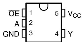
图 5-1. SN74AHC1G125-Q1 DBV Package, 5-Pin SOT-23; DCK Package, 5-Pin SC-70 (Top View)
