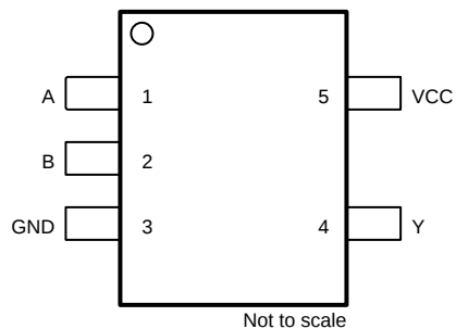
图 5-1. SN74AHC1G02-Q1 DBV Package, 5-Pin SOT-23; DCK Package, 5-Pin SC-70 (Top View)
