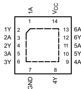
图 4-2. RGY or BQA Package, 14-Pin VQFN or WQFN (Top View)
