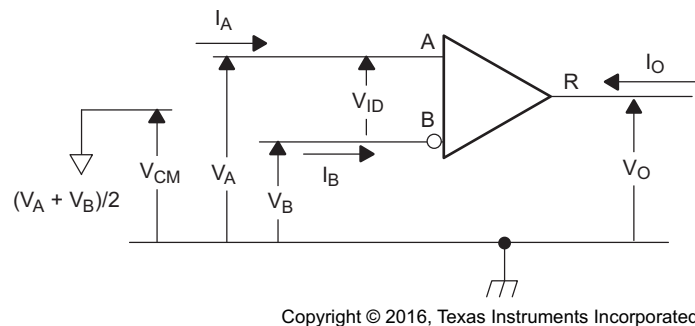
图 10. Receiver Voltage and Current Definitions
