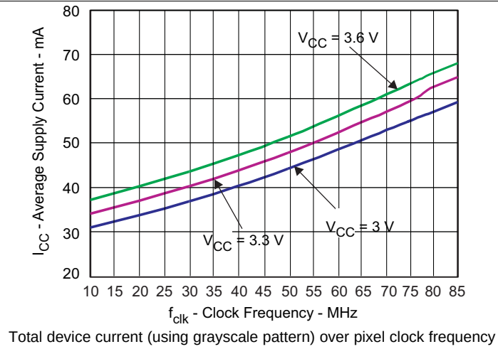
图 2. Average Grayscale ICC vs Clock Frequency
