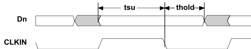
Figure 6. Set Up and Hold Time Definition
