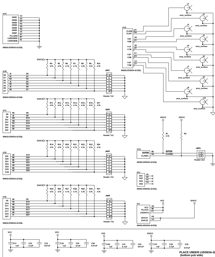
Figure 14. Schematic Example (SN65LVDS93A-Q1 Evaluation Board)
