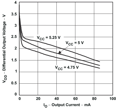
图 5-1. Differential Output Voltage vs Output Current
