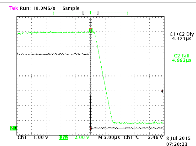
图 10-3. Recessive-to-Dominant Propagation Delay
