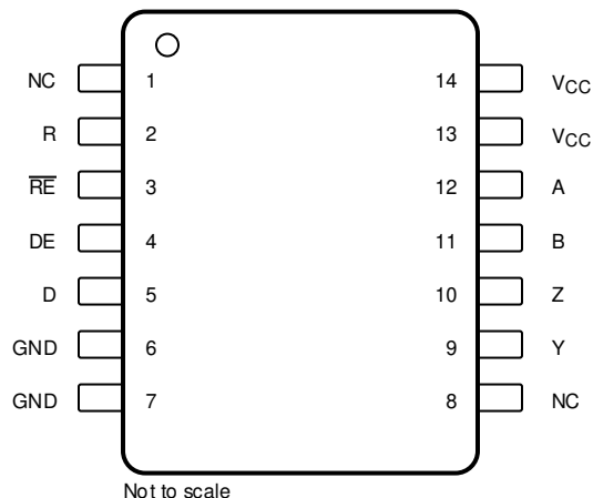
SN65HVD70, SN65HVD73, SN65HVD76 14-Pin SOIC, D Package (Top View)
