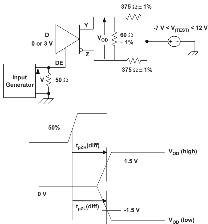
图 7-12. Driver Enable Time From DE to V OD
