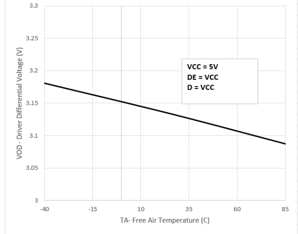
图 7-8. Driver Differential Output Voltage vs Free-Air Temperature
