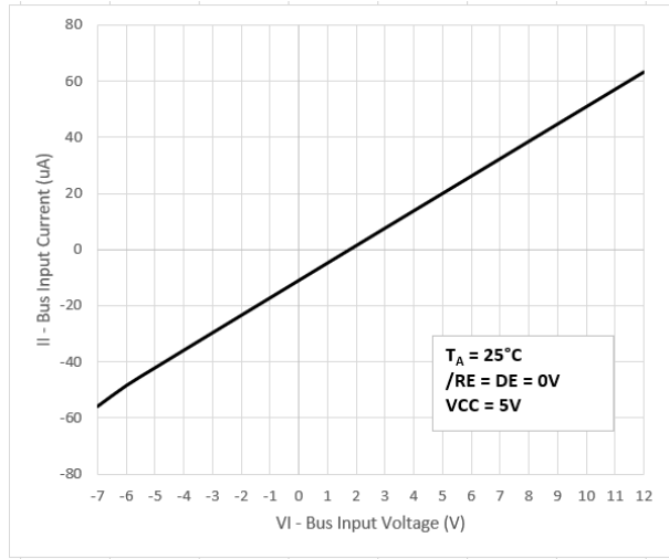
图 7-5. HVD51, HVD52, HVD54, HVD55 BUS Input Current vs Input Voltage
