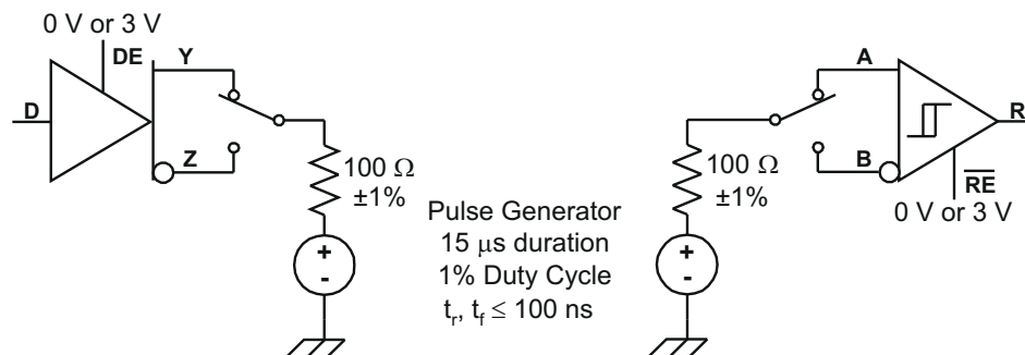
图 8-12. Test Circuit, Transient Overvoltage Test
