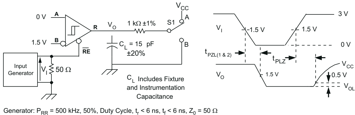
图 8-11. Receiver Low-Level Enable and Disable Time Test Circuit and Voltage Waveforms
