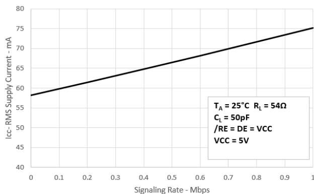
图 7-3. HVD52, HVD55 RMS Supply Current vs Signaling Rate
