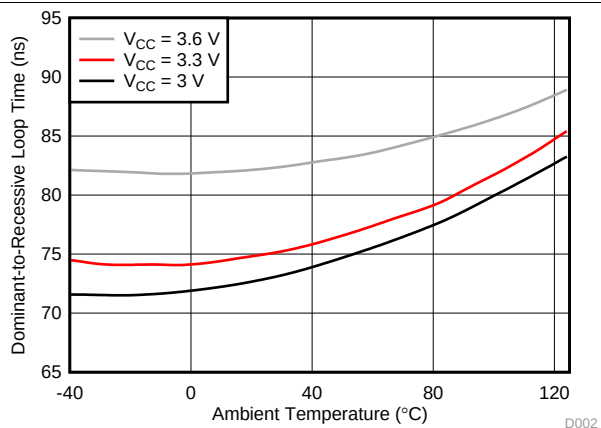
Figure 2. Dominant-to-Recessive Loop Time vs Ambient Temperature
