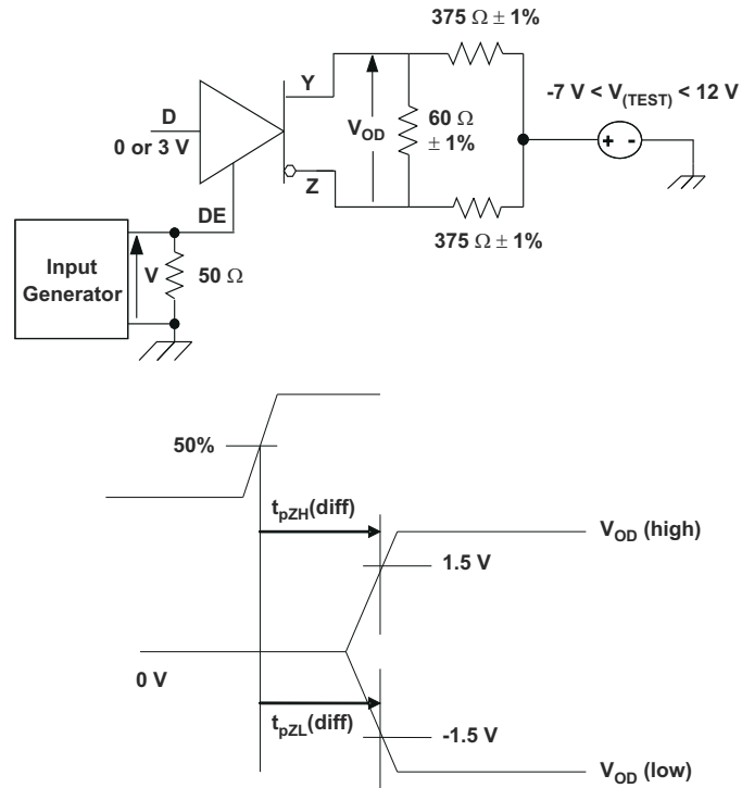
图 6-1. Driver Enable Time From DE to V OD
