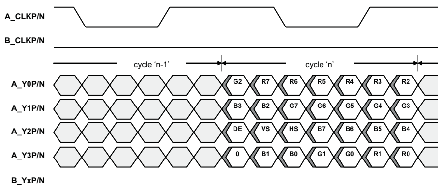
Figure 11. Flatlink Output Data (Format 1); Single-Link 24 Bpp
