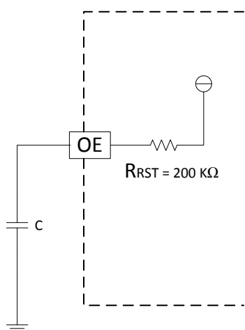
图 19. External Capacitor Controlled OE
