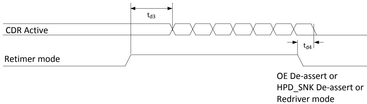
图 22. CDR Timing for SNx5DP149
