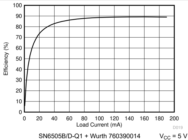
图 6-22. Efficiency vs Load Current
