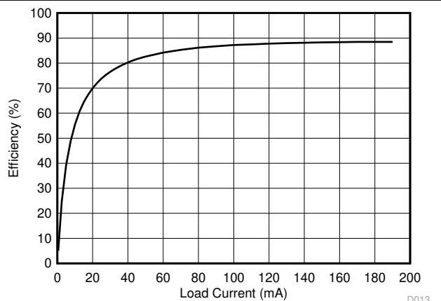
图 6-14. Efficiency vs Load Current
