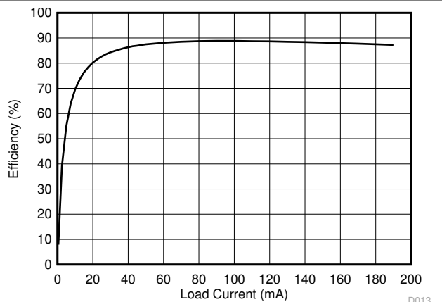
图 6-18. Efficiency vs Load Current
