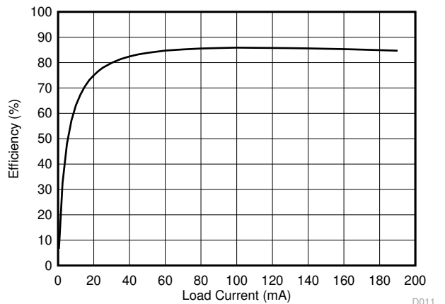
图 6-12. Efficiency vs Load Current
