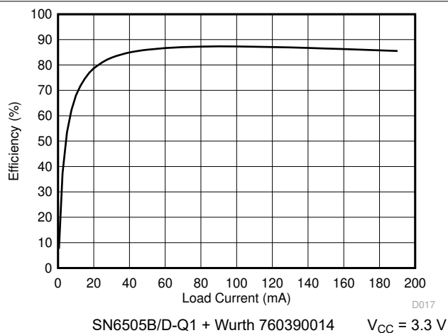
图 6-20. Efficiency vs Load Current
