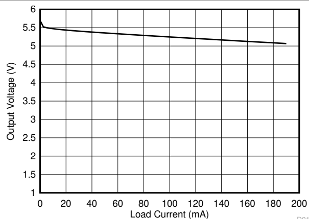
图 6-17. Output Voltage vs Load Current
