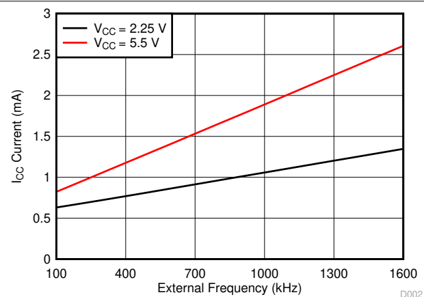
图 6-46. Current vs External Frequency
