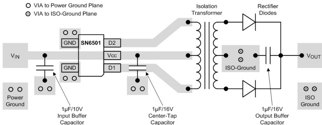
图 11-1. Layout Example of a 2-Layer Board (SN6501)
