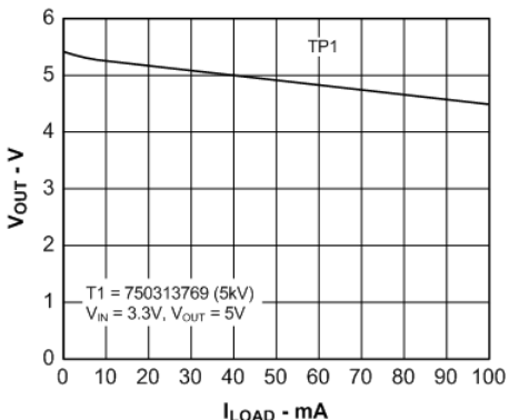
图 6-19. Output Voltage vs Load Current
