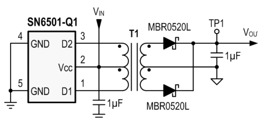
图 9-6. Unregulated Output for Low-Current Loads With Wide Supply Range
