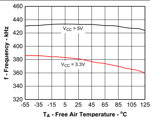
图 6-30. D1, D2 Switching Frequency vs Free-Air Temperature
