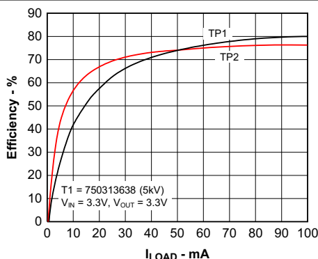
图 6-22. Efficiency vs Load Current
