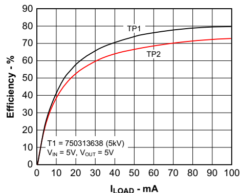
图 6-24. Efficiency vs Load Current
