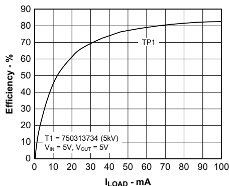
图 6-18. Efficiency vs Load Current
