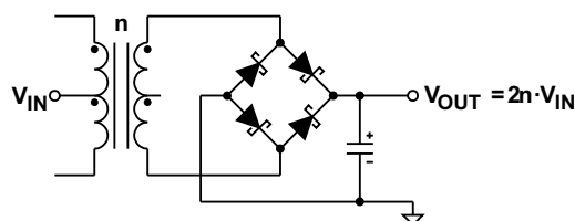
图 9-9. Bridge Rectifier Without Center-Tapped Secondary Performs Voltage Doubling
