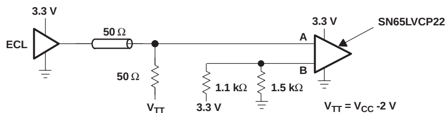
Figure 23. Single-Ended (LVPECL)
