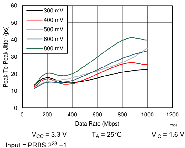
图 6-9. Peak-To-Peak Jitter vs Data Rate
