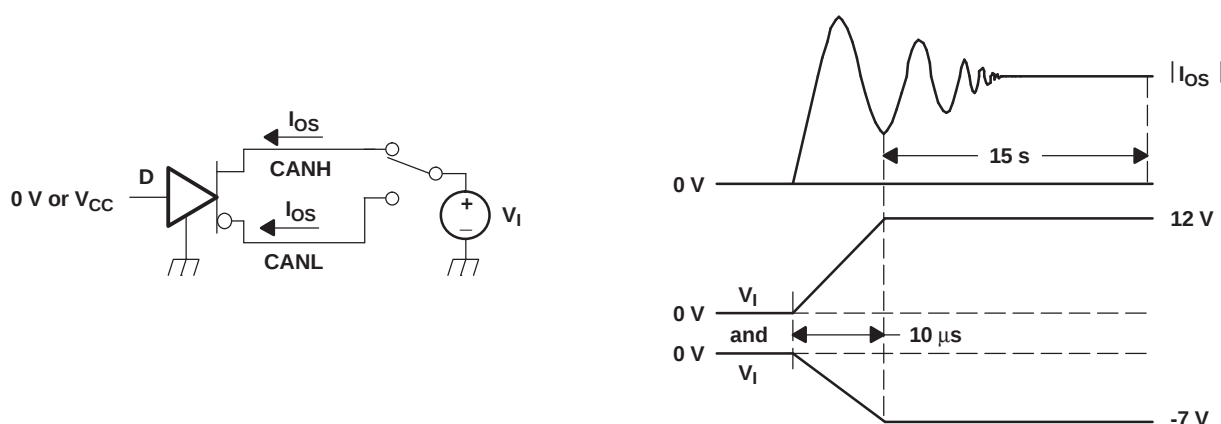
Figure 23. I_{OS} Test Circuit and Waveforms
