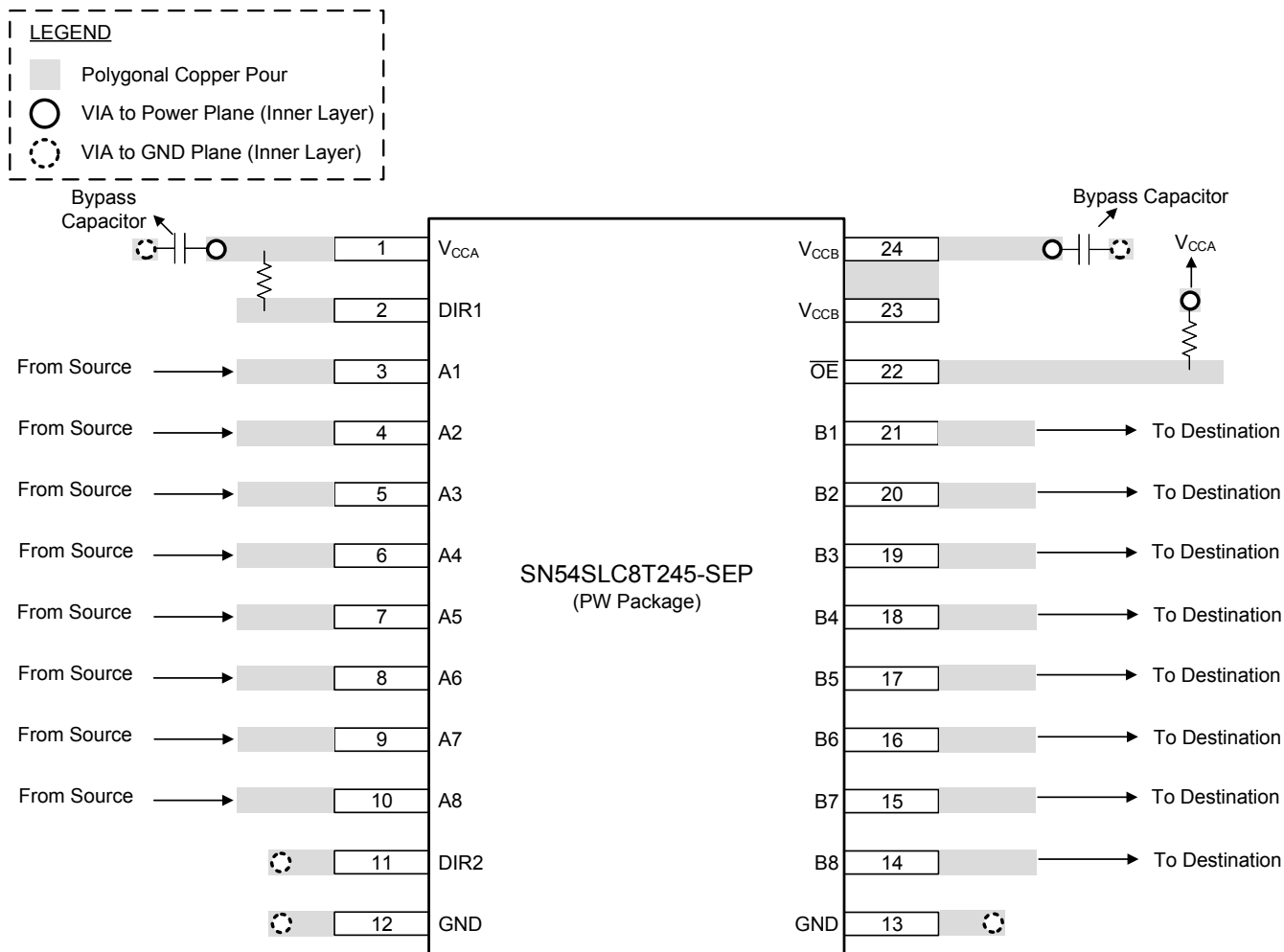
图 8-3. SN54SLC8T245-SEP Device Layout Example
