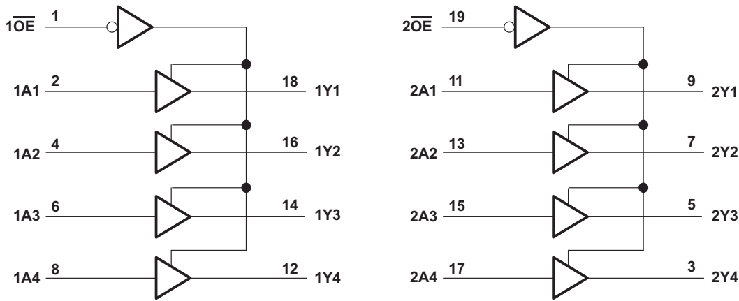
图 7-1. Logic Diagram (Positive Logic)
