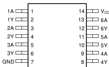
图 4-1. D, DB, N, NS, PW, J, or W Package 14-Pin SOIC, SSOP, PDIP, SO, TSSOP, CDIP, or CFP Top View
