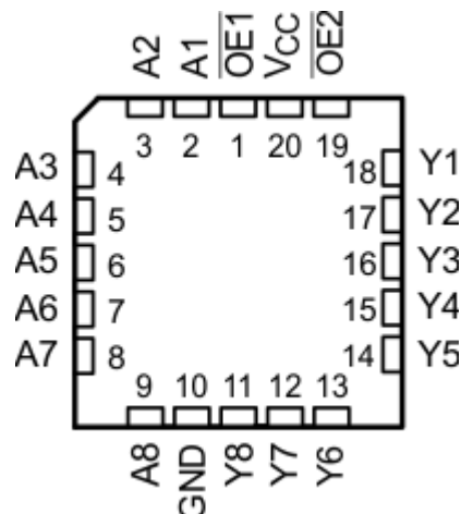
图 3-2. SN54AHCT541 FK Package, 20-Pin LCCC (Top View)
