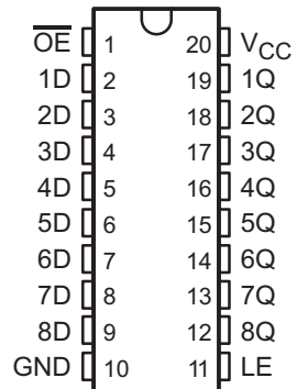
SN54AHC573 . . . J OR W PACKAGE SN74AHC573 . . . DB, DGV, DW, N, NS, OR PW PACKAGE (TOP VIEW)
