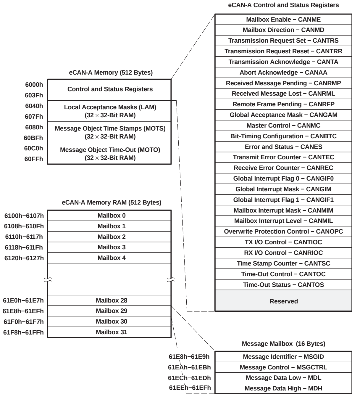
Figure 4-13. eCAN-A Memory Map
