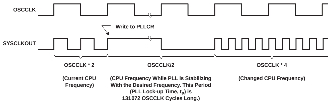
Figure 6-9. Example of Effect of Writing Into PLLCR Register
