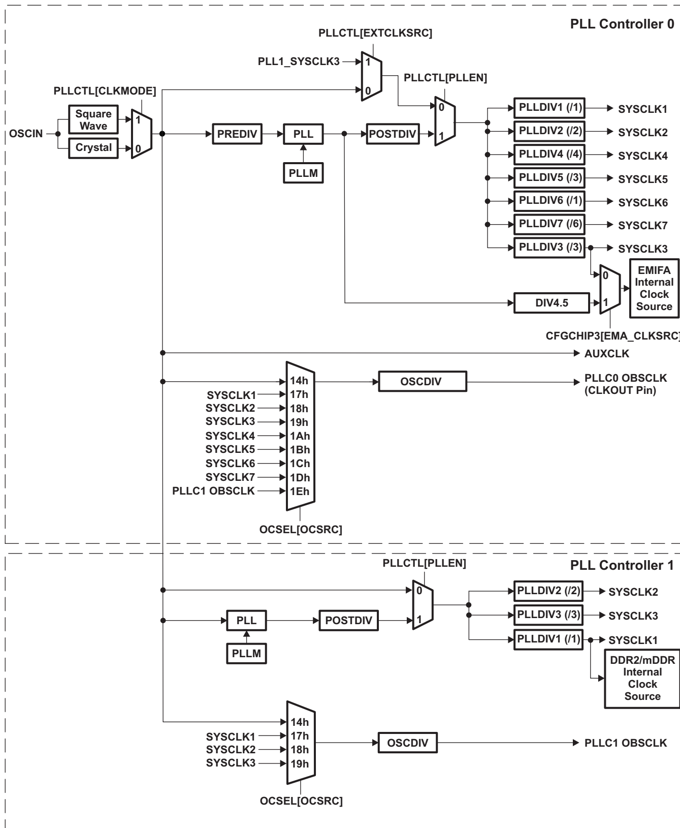
Figure 4-10. PLL Topology
