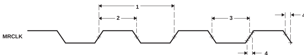
Figure 7-48. MRCLK Timing
