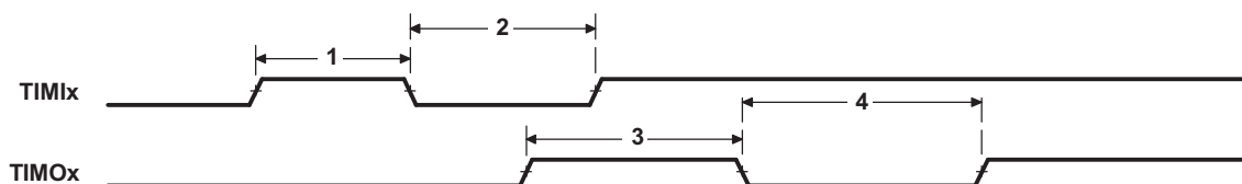
Figure 4-61. Timer Timing
