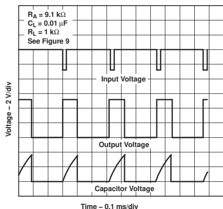
图 6-3. Typical Monostable Waveforms
