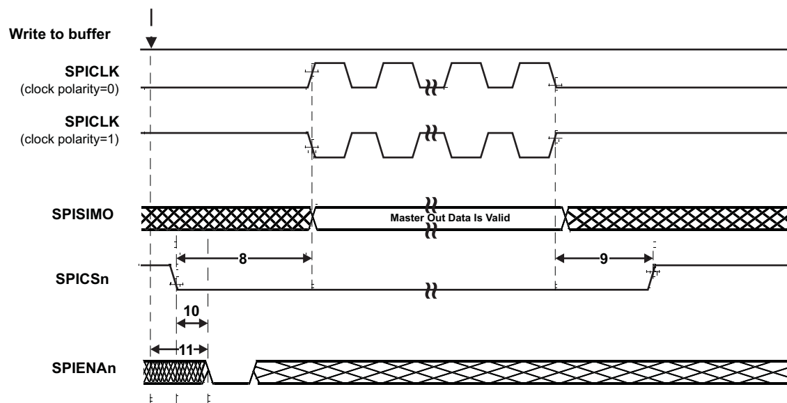
图 7-21. SPI Master Mode Chip Select Timing (CLOCK PHASE = 1)
