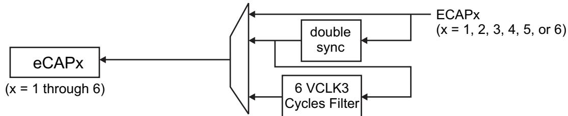
图 7-5. eCAPx Input Synchronization Selection Detail
