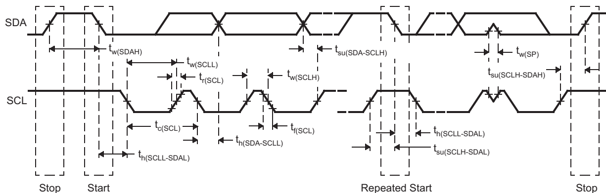
图 7-17. I2C Timings
