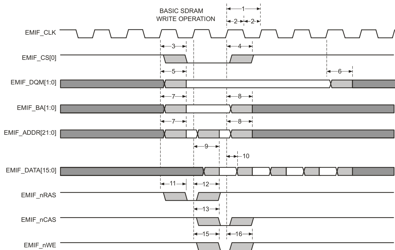
图 6-16. Basic SDRAM Write Operation
