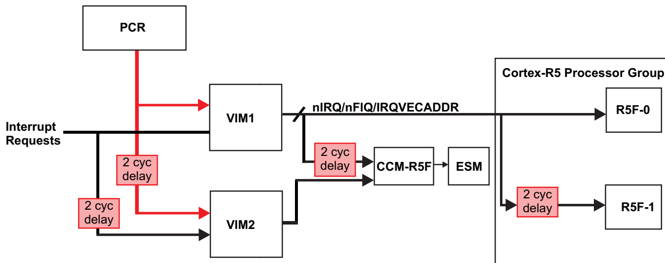
图 6-17. Interrupt Generation
