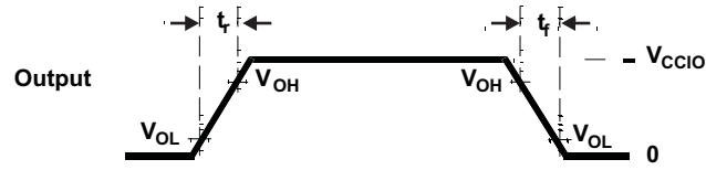
Figure 3-3. CMOS-Level Outputs
