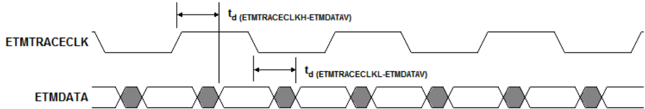
Figure 4-23. ETMDATA Timing
