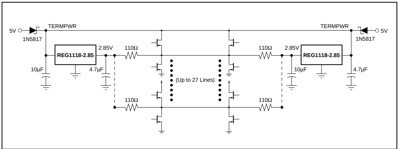
FIGURE 3. SCSI Active Termination Configuration.
