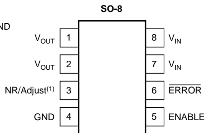
(U Package)
