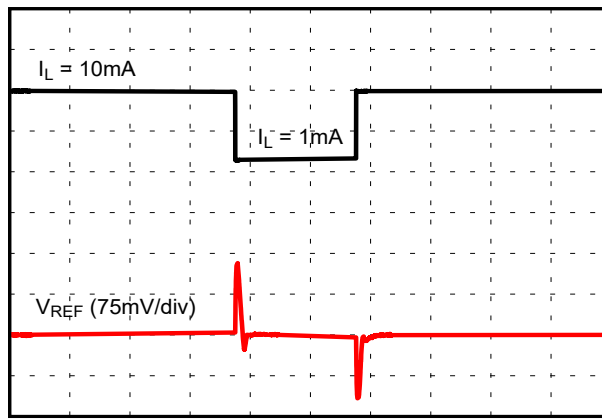
图 9-4. Load Transient Response 1 mA to 10 mA, C_{REF} = 1 \mu F
