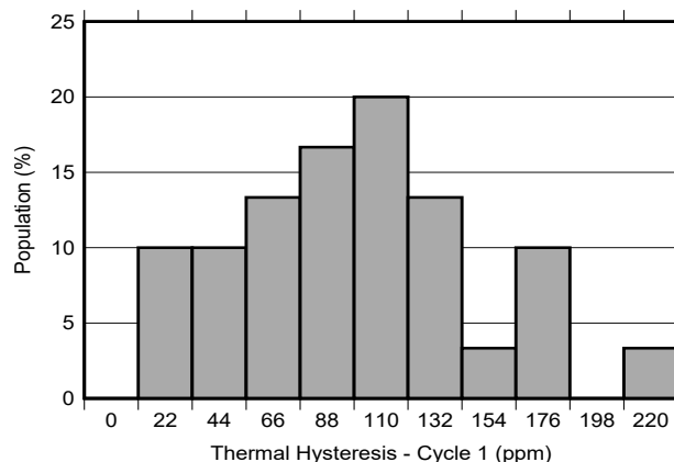
图 8-5. Thermal Hysteresis Distribution -40°C to 125°C, Cycle 1
